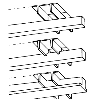
12 Floor slab supports, double-T
